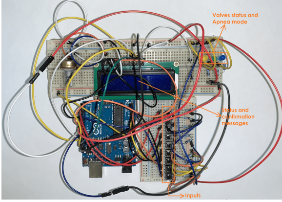
Figure 5: The Arduino version of the MVM
