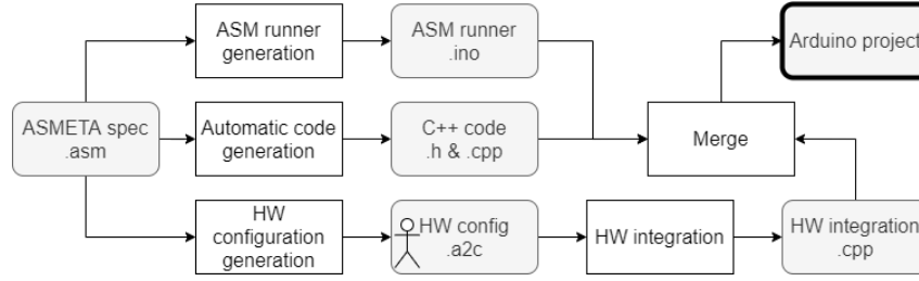
Figure 4: Arduino code generation process
