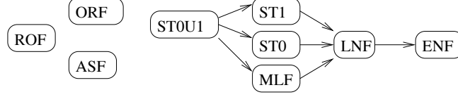
Fig. 1. boolean fault hierarchy
